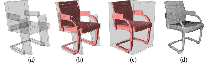
Fig. 14. Geometry synthesis from part structure. Given a generated part structure (a), we synthesize the geometry inside each part box in volumetric representation (b). The per-box volumes are then embedded into a global volume (c) from which we reconstruct the final meshed model (d).
