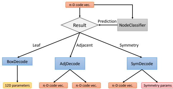
Fig. 5. Autoencoder test decoding setup.
