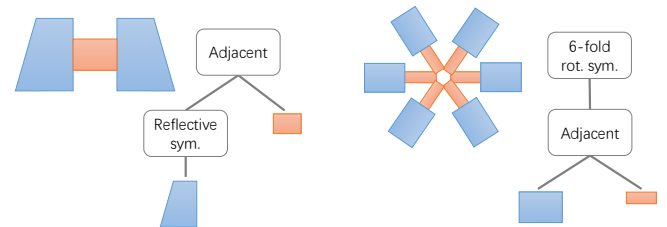
Fig. 6. Different two-step encoding orders for two examples, found by minimizing reconstruction errors during testing. Left: Symmetry (reflective) before adjacency. Right: Adjacency before symmetry (6-fold rotational).
