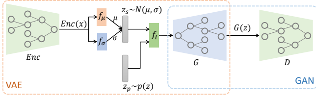
Fig. 11. Confining random codes by sampling from a learned Gaussian distributions based on learned root codes Enc(x) . Jointly learning the distribution and training the GAN leads to a VAE-GAN network.
