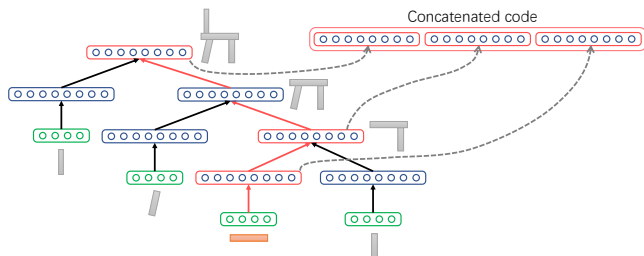
Fig. 12. Construction of structure-aware recursive feature (SARF) for a part in a hierarchy. We concatenate the RvNN codes of the part, its immediate parent, and the root into a fixed-dimensional vector.
