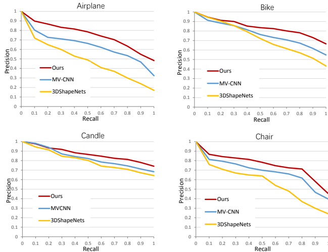
Fig. 17. Precision-recall plots for classification tasks.
